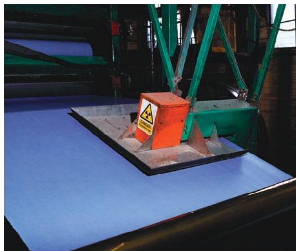
Figure 49.11 Quality control in the manufacture of paper using a radioactive gauge
