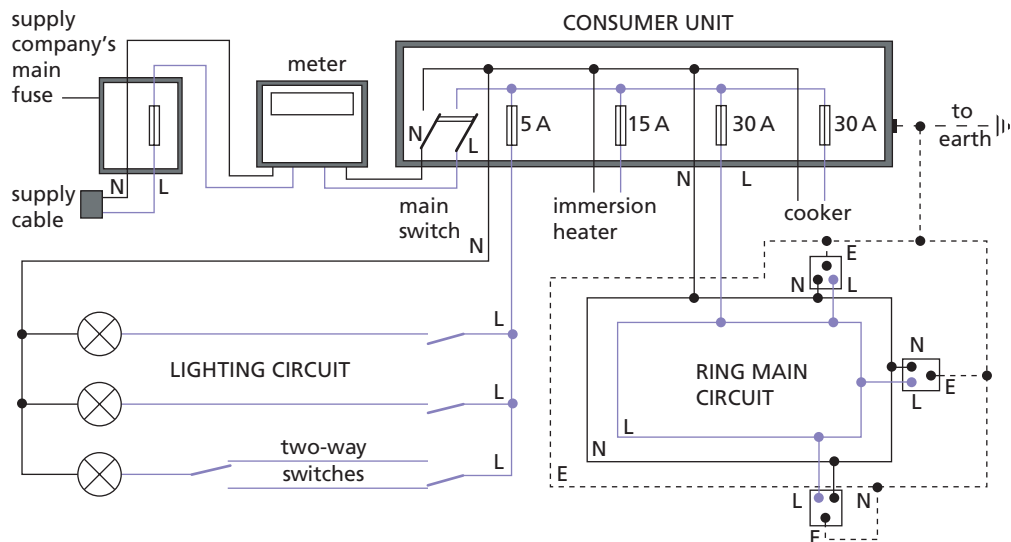
Figure 40.9 Electric circuits in a house
